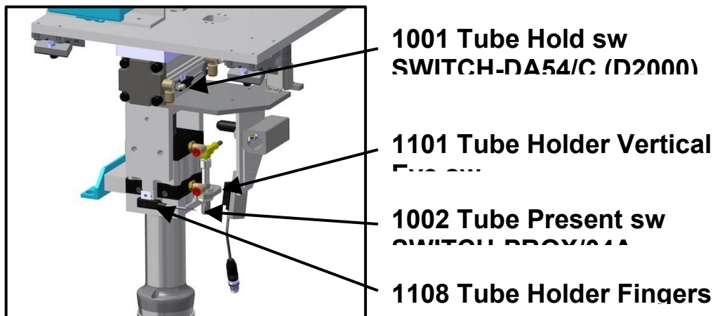
Figure 9- Tube Holder, Tube Holder Vertical Eye
