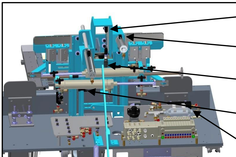
Figure 18 - Box Fold Back/Table Box Hold Vacuum Switch
