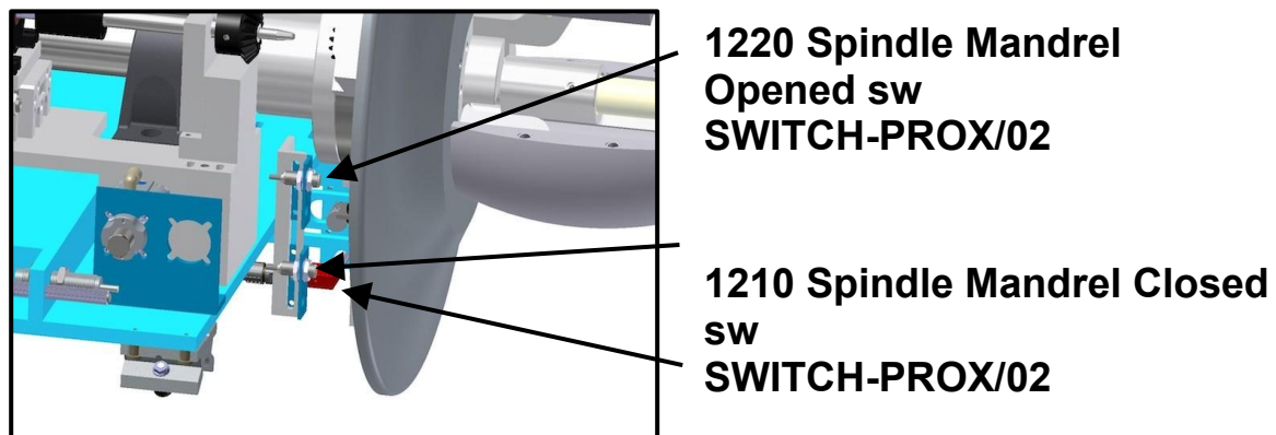
Figure 7 - Spindle Mandrel
