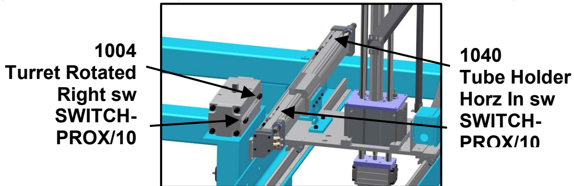
Figure 4- Turret Rotary Actuator, Tube Holder Horizontal Cylinder
