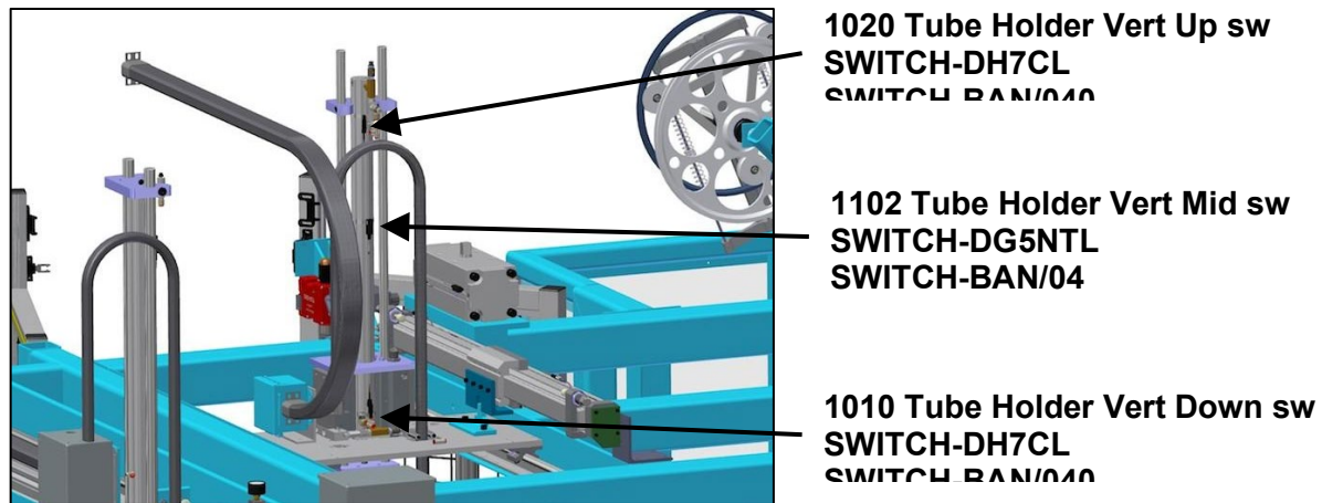
Figure 10 - Tube Holder Vertical Cylinder
