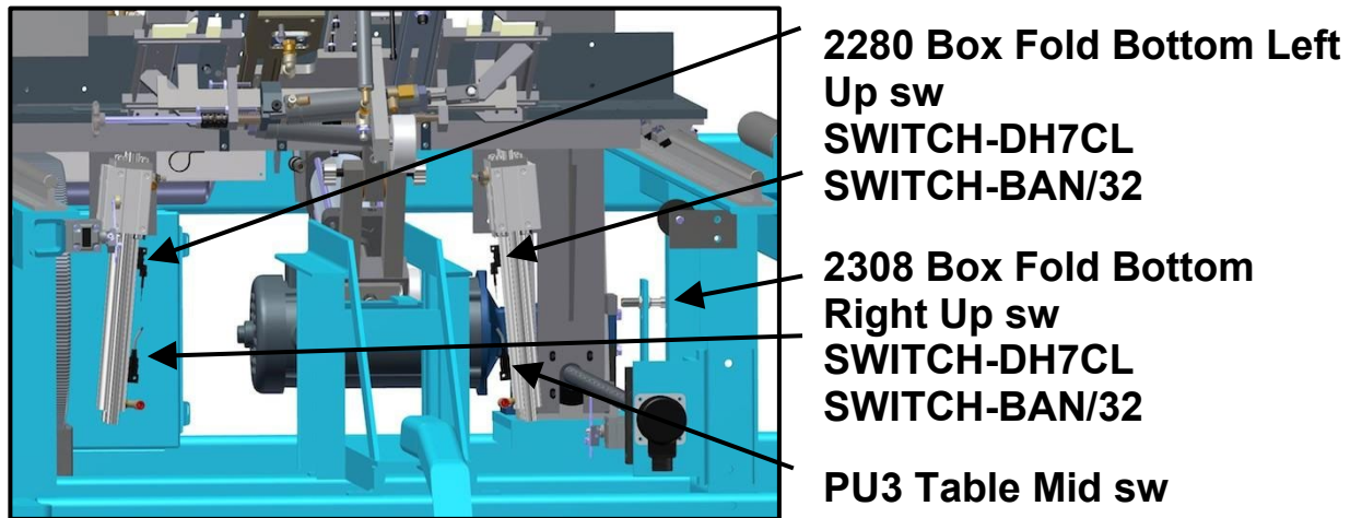
Figure 21 - Compression Cylinder
