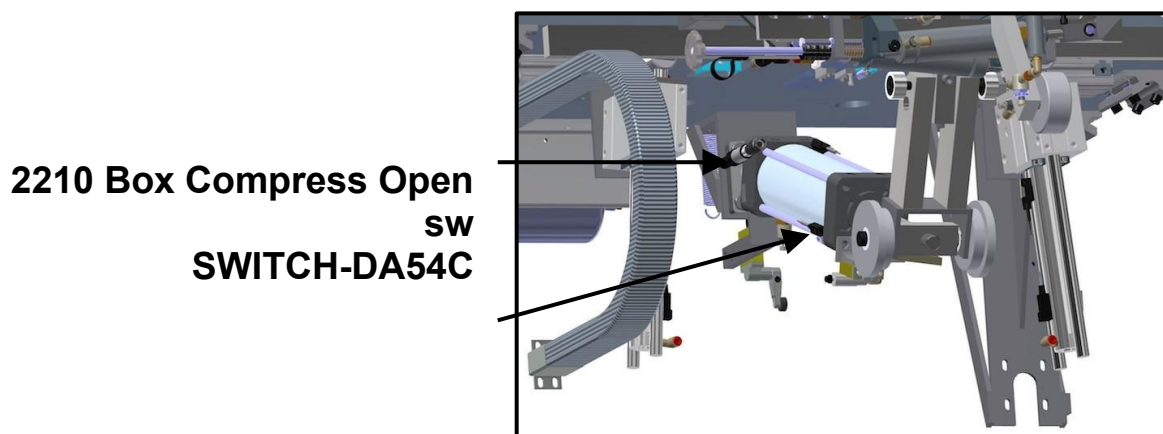
Figure 22 - Conveyor
