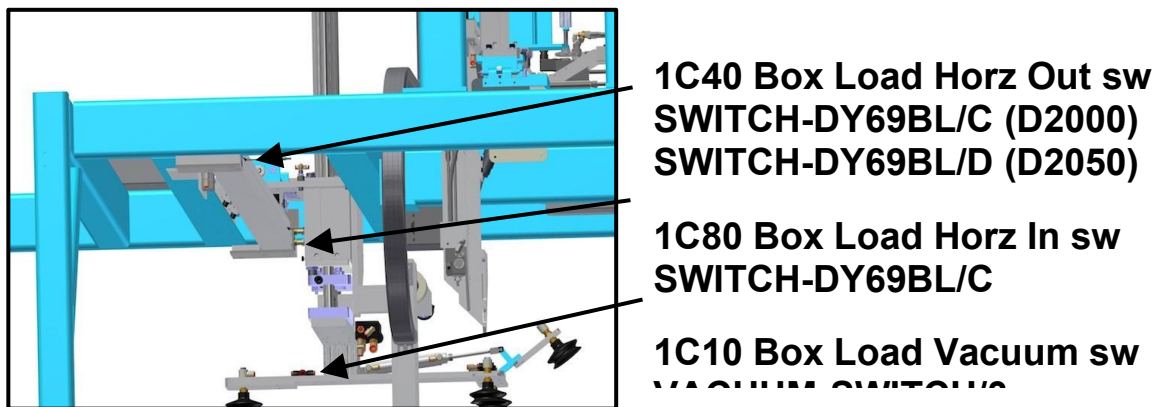
Figure 14 - Box Load Horizontal Cylinder
