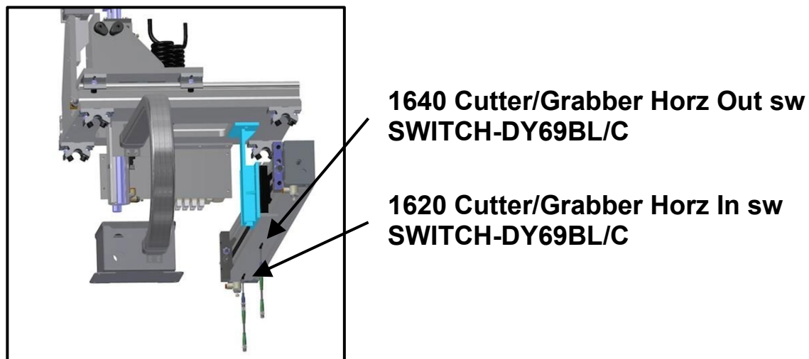
Figure 23 - Robot Arm (D-2050 Only)
